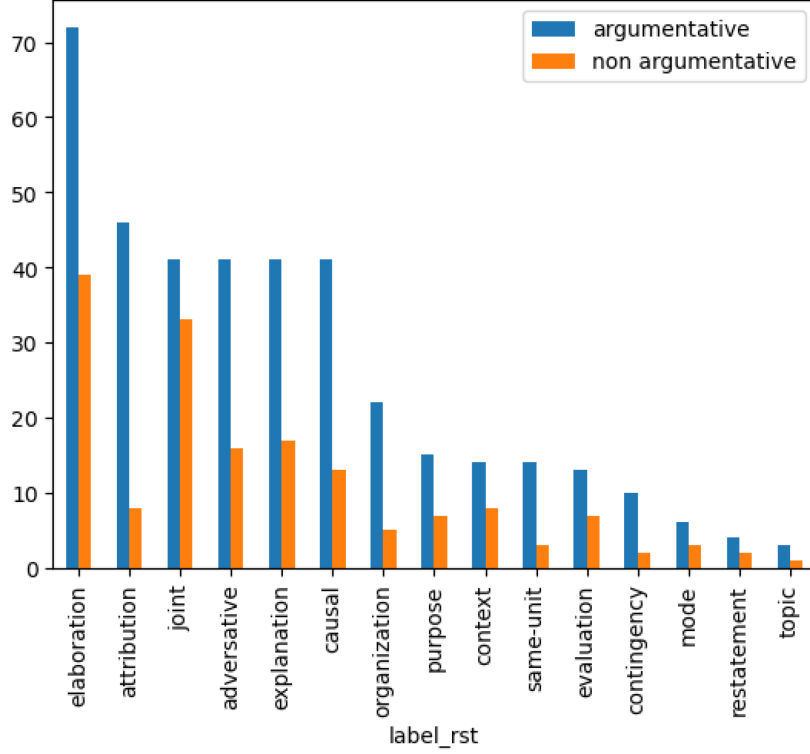
Figure 3: Rhetorical relations between positive pairs of statements (connected by argumentative relations) and negative ones
