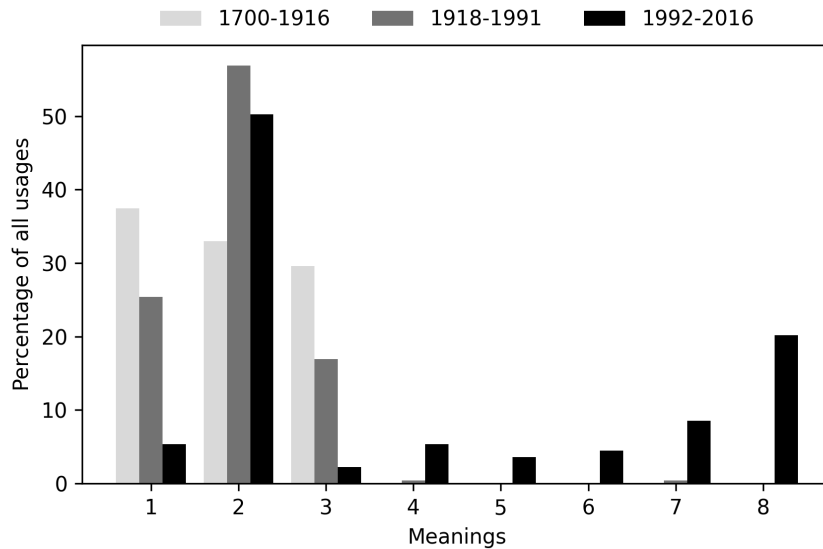
Figure 2: Semantic Shift of the Word nakem [ bag/package ] (Parameters: \text{eps}=0.11 , \text{min\_samples}=8 )
